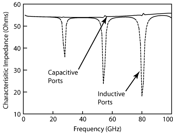
Fig. 6. When the L -length standard is a multiple of a half-wavelength long, there is difficulty deembedding both shunt capacitive (shielded) and series inductive (unshielded) port discontinuities.
