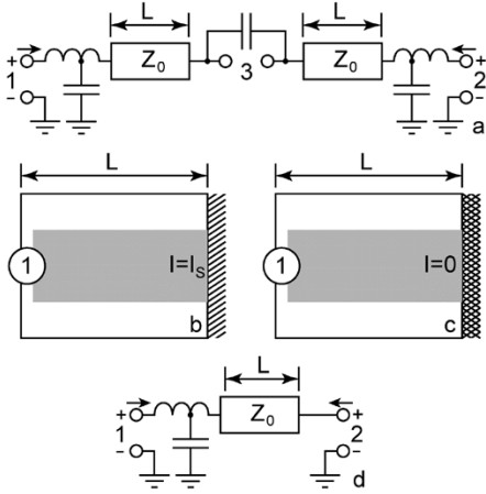
Fig. 3. Circuit theory model of the SOC standard: (a) includes arbitrary reciprocal port discontinuities. By exciting ports 1 and 2 symmetrically and antisymmetrically either: (b) an electric wall or (c) magnetic wall can be placed at the location of port 3. This allows characterization of a single-port discontinuity plus (d) connecting transmission line.
