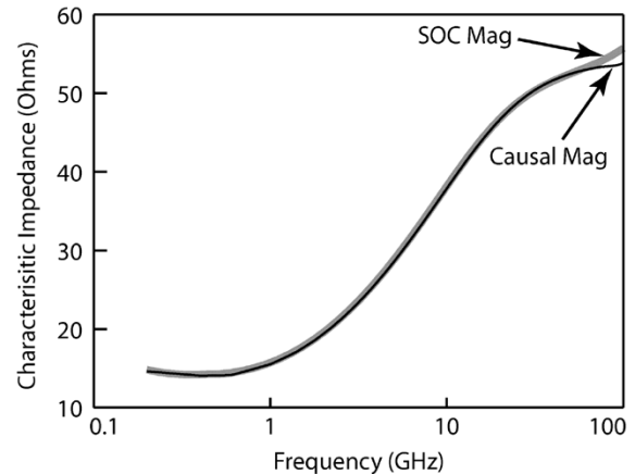
Fig. 5. Phase of the SOC calculated characteristic impedance is used to calculate the magnitude required for causality and is compared to the SOC calculated magnitude for a lossy line.
