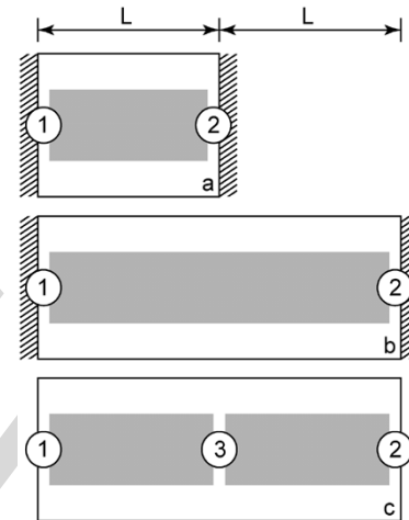
Fig. 1. Double-delay calibration uses: (a) an L -length and (b) a 2L -length through line. The ports must be backed by a perfectly conducting electric wall. The SOC uses: (c) a single three-port 2L -length standard. Perfect ground reference is not needed.
