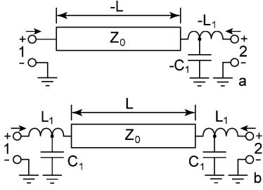
Fig. 4. Extending the SOC to calculate the naked port discontinuity without the port connecting line, invert the ABCD matrix of the circuit of Fig. 3(d), yielding (a), and cascade it with an L length through, as shown in (b).
